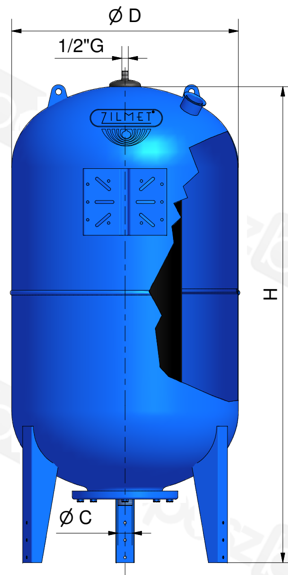
VERTICAL MODEL
