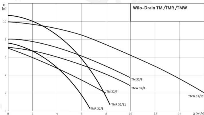
Jelleggörbék Wilo-Drain TM/TMR/TMW 32 - 50 Hz - 2900 1/min
