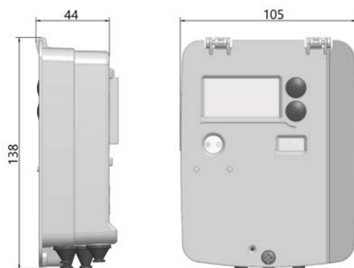
Fig. 1: Dimensions Processor
