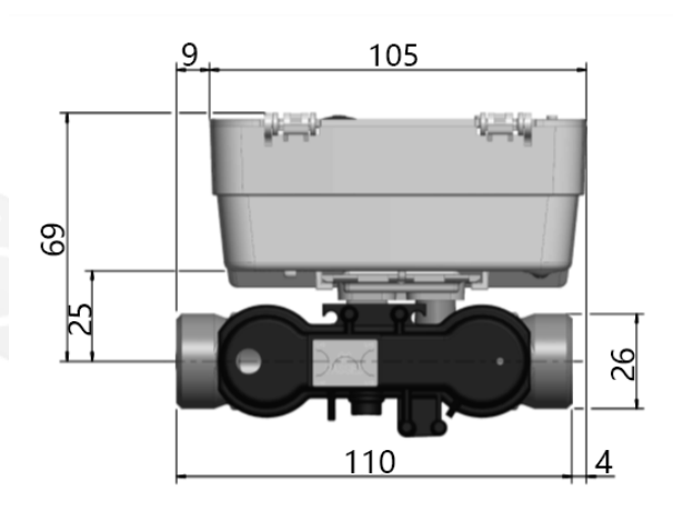
Fig. 3: Overview of dimensions mounting length 110 mm
