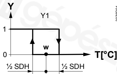
Heating and cooling mode (P01=04)
