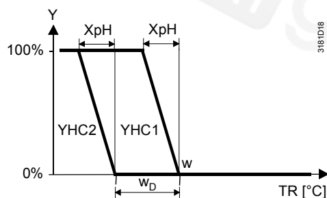
Changeover (P01=2 or P01= 3)
