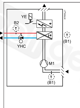
2-pipe fan coil unit with electric heater
