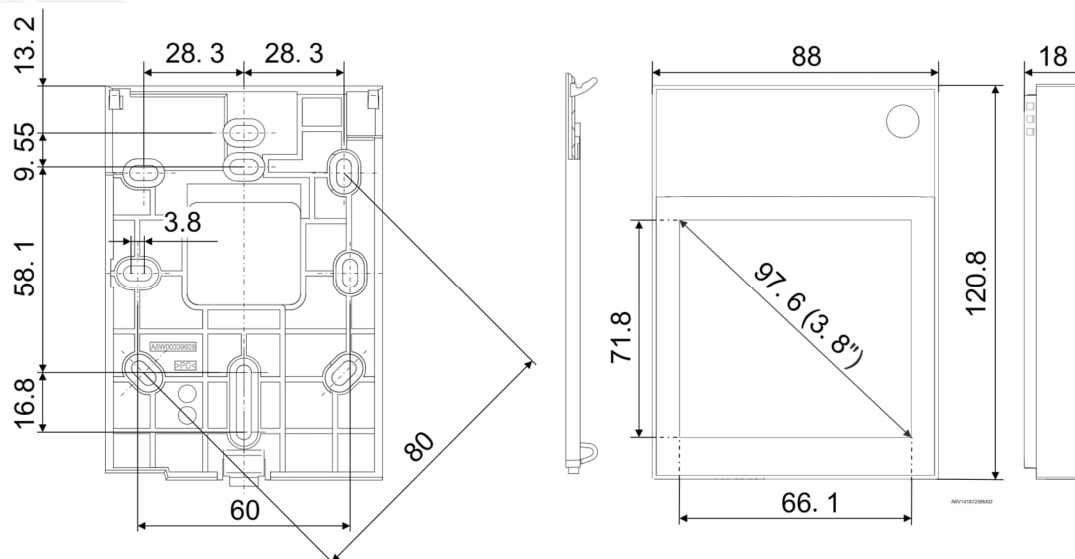
Fig. 4: Dimension drawing
