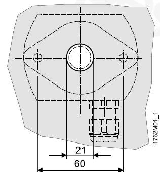
Drilling plan
