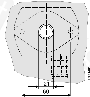
Drilling plan
