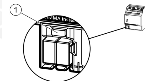
Fig. 2: Programming button and programming LED (exemplary illustration)
