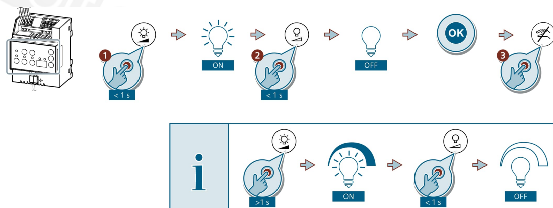
Fig. 11: KNX/DALI Gateway - testing the DALI broadcast
