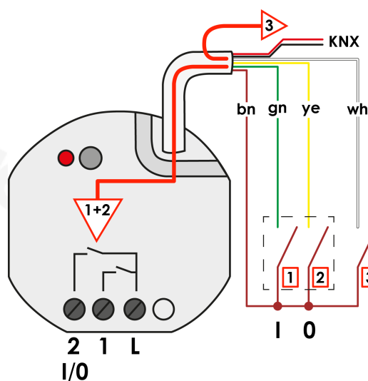
Image 28: Functionality of the inputs when controlling the internal switching output 2 as two-area operation
