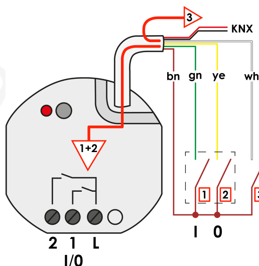
Image 27: Functionality of the inputs when controlling the internal switching output 1 as two-area operation
