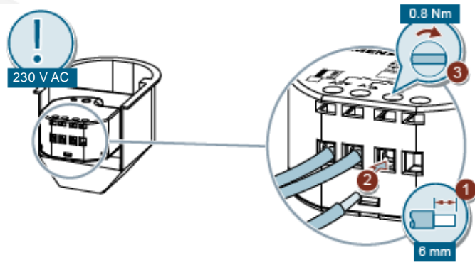
Fig. 3: Connecting loads to the switching contact
