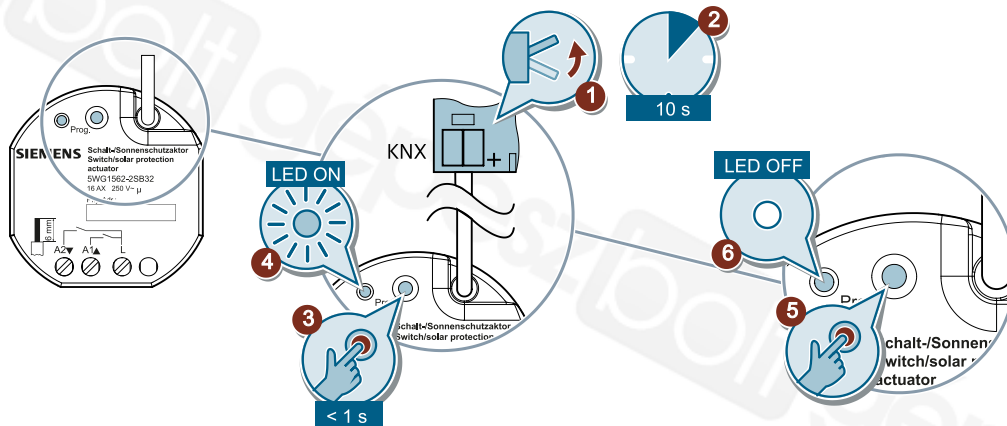
Fig. 4: Test of KNX 24 V DC type SELV
