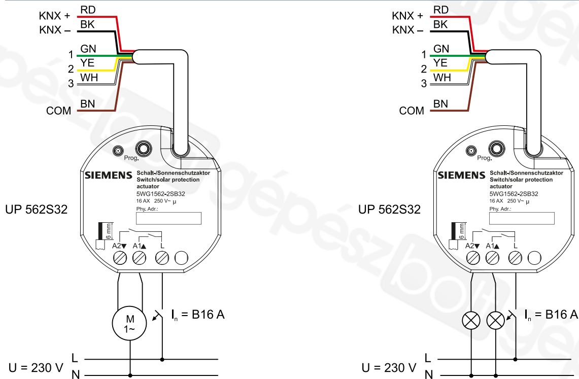
Fig. 7: Connection examples for switching outputs and solar protection control
