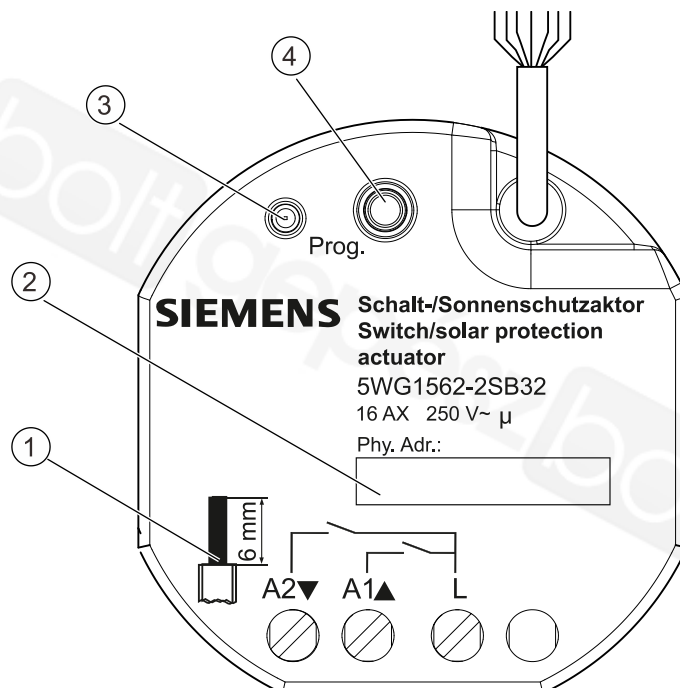
Fig. 2: Connections, operating and display elements
