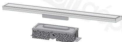
uBox + Original
