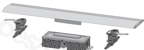
uBox + Match/Rock
