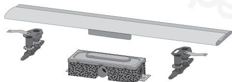
uBox + Match
