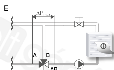
Circuit with local circulation pump
