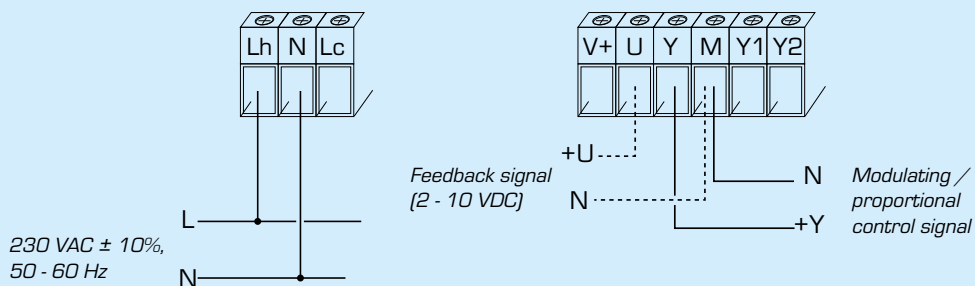
Modulating / proportional control mode
