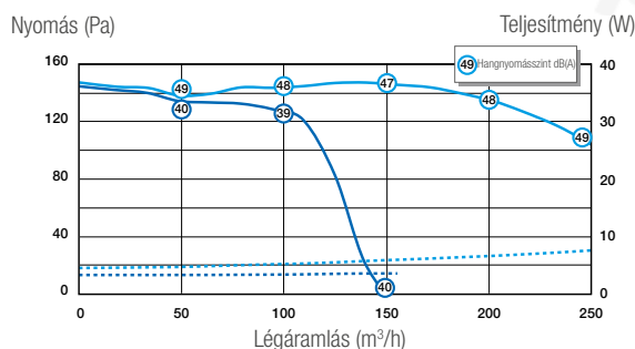
Jelleggörbék
